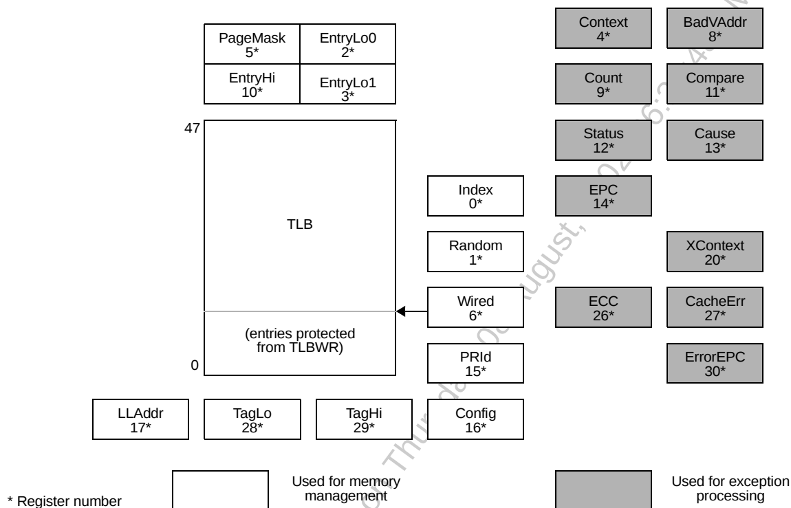
Figure 4 CP0 Registers
