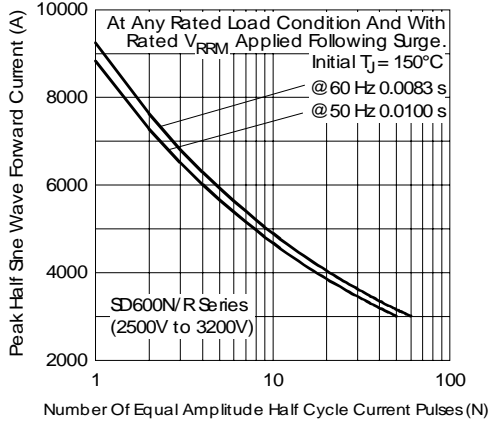
Fig. 11 - Maximum Non-Repetitive Surge Current
