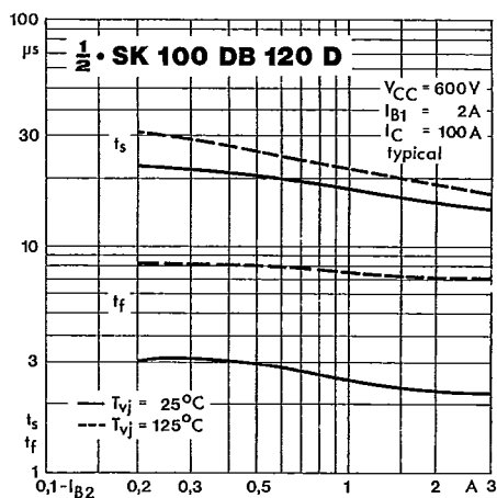
Fig. 10 Turn-off times vs. negative base current
