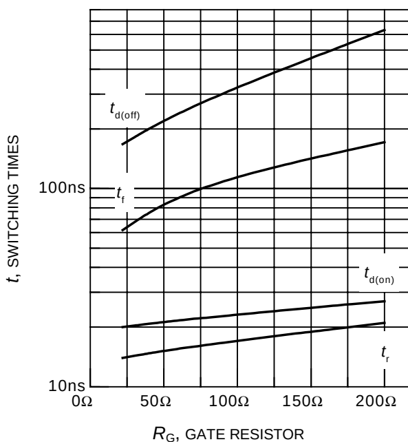
Figure 10. Typical switching times as a function of gate resistor
