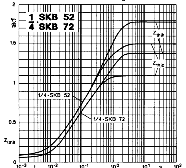
Fig. 12 a Transient thermal impedance vs. time
