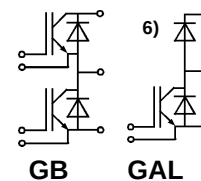
SEMITRANS 2N (low inductance)
