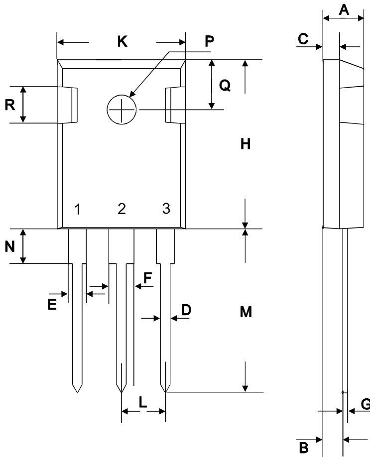
TO-247AC
