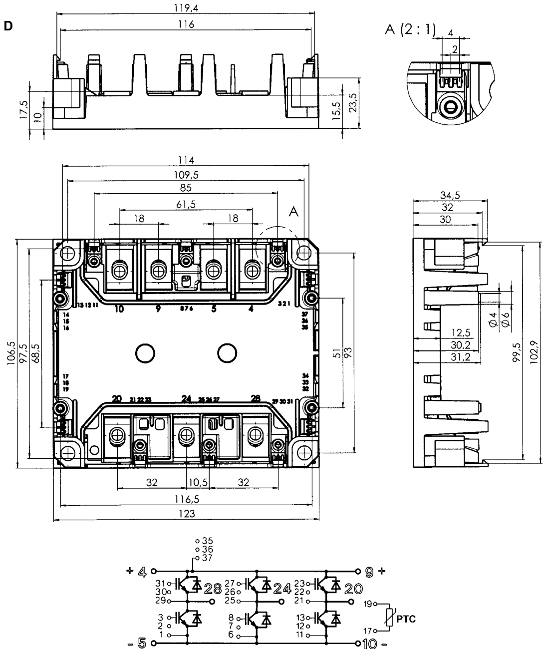
Case outline and circuit diagram
