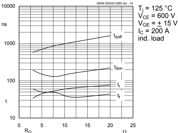
Fig. 14 Typ. switch times vs. gate resistor R_G
