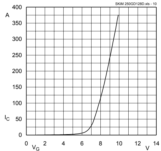
Fig. 10 Typ. transfer characteristic, t p = 80 μs; VCE = 20 V
