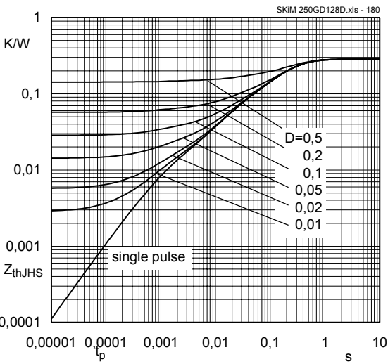
Fig. 18 Transient thermal impedance of inverse CAL diodes Z_{thJHS} = f(t_p) ; D = t_p / t_c = t_p \cdot f
