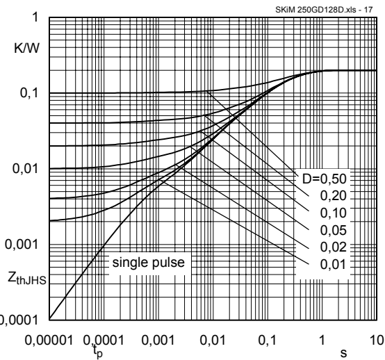
Fig. 17 Transient thermal impedance of IGBT Z_{thJHS} = f(t_p) ; D = t_p / t_c = t_p \cdot f
