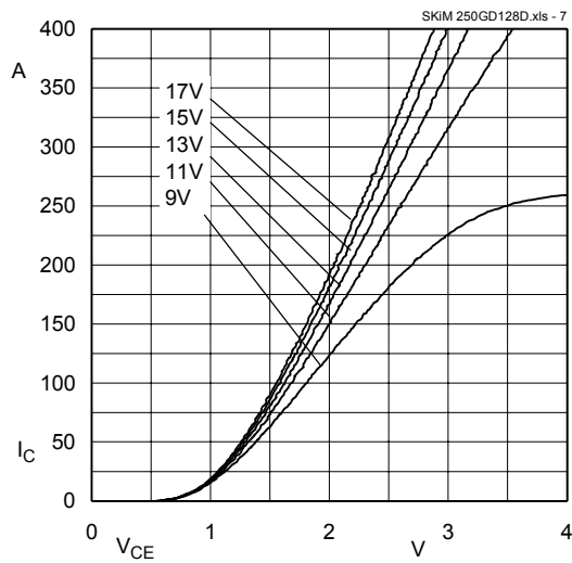
Fig. 7 Typ. output characteristic, t p = 80 μs; 25 °C
