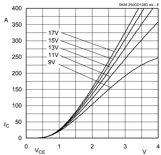
Fig. 8 Typ. output characteristic, t p = 80 μs; 125 °C
