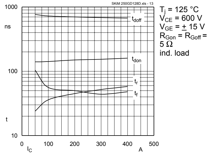
Fig. 13 Typ. switch times vs. I_C
