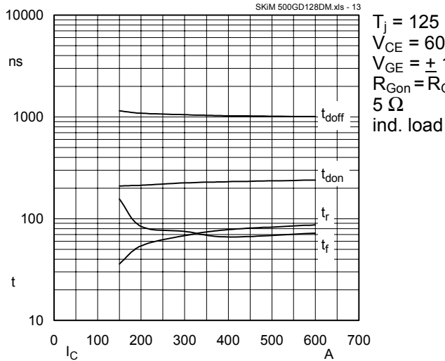
Fig. 13 Typ. switch times vs. I_C
