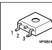
P-TO263-3-2
